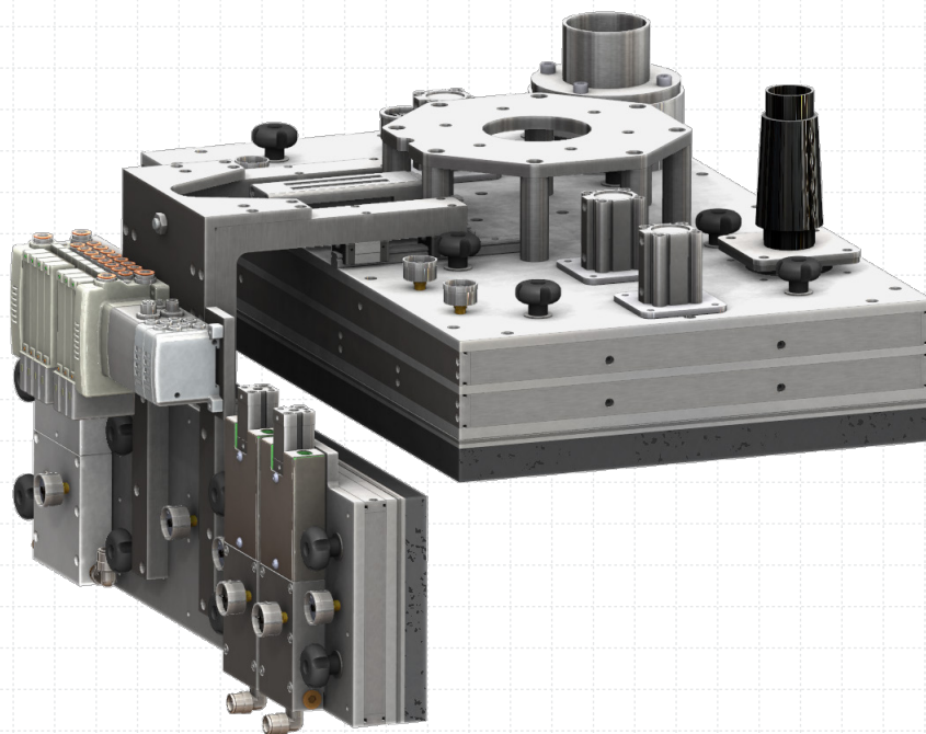
Linear side gripper with separate vacuum source
